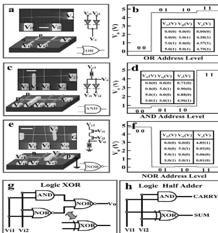
Fig 3: Nanoscale logic gates.
